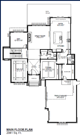
Main Floor
